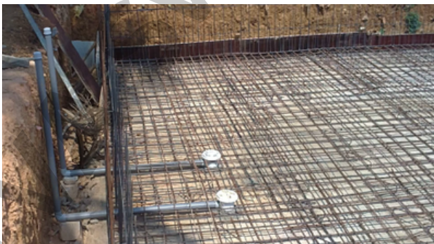
FLOOR PIPING
